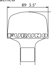
GPS/WAAS Receiver Antenna GP-320B 0.8 kg 1.8 lb 10 m cable attached
