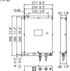
Network Weather Facsimile Receiver FAX-30 2.0 kg 4.4 lb
