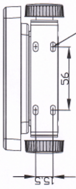
BOTTOM VIEW
