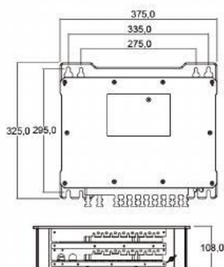
Distribution Processor
