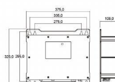
Transceiver Unit
